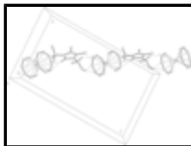
Fig. 2. Chain formation via short C—H... \pi contacts (thin dashed bonds) - see text. H atoms not involved in short contacts are omitted for clarity.
